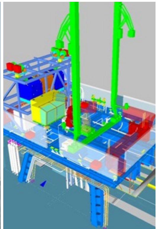
3D-model, structure | Illustration: Multiconsult
